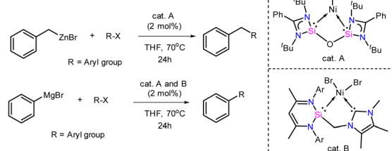
Chart 4 Previous reports on C–C coupling reactions with NHSi as a ligand on the metal centre. (cod = cyclooctadiene).
