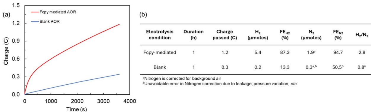
Fig. 3 (a) Constant potential electrolysis at 0.28 V (vs. \text{Fc}^{+/0} ) for the same duration without (blue) and with (red) 1 mM Fcpy using 1 \times 1 \text{ cm}^2 carbon-cloth as working electrode. Experimental conditions: 100 mM TBAF as supporting electrolyte in acetonitrile, 3-electrode setup in an undivided cell, 298 K; (b) summary of product quantification results after electrolysis with an average of three measurements.
