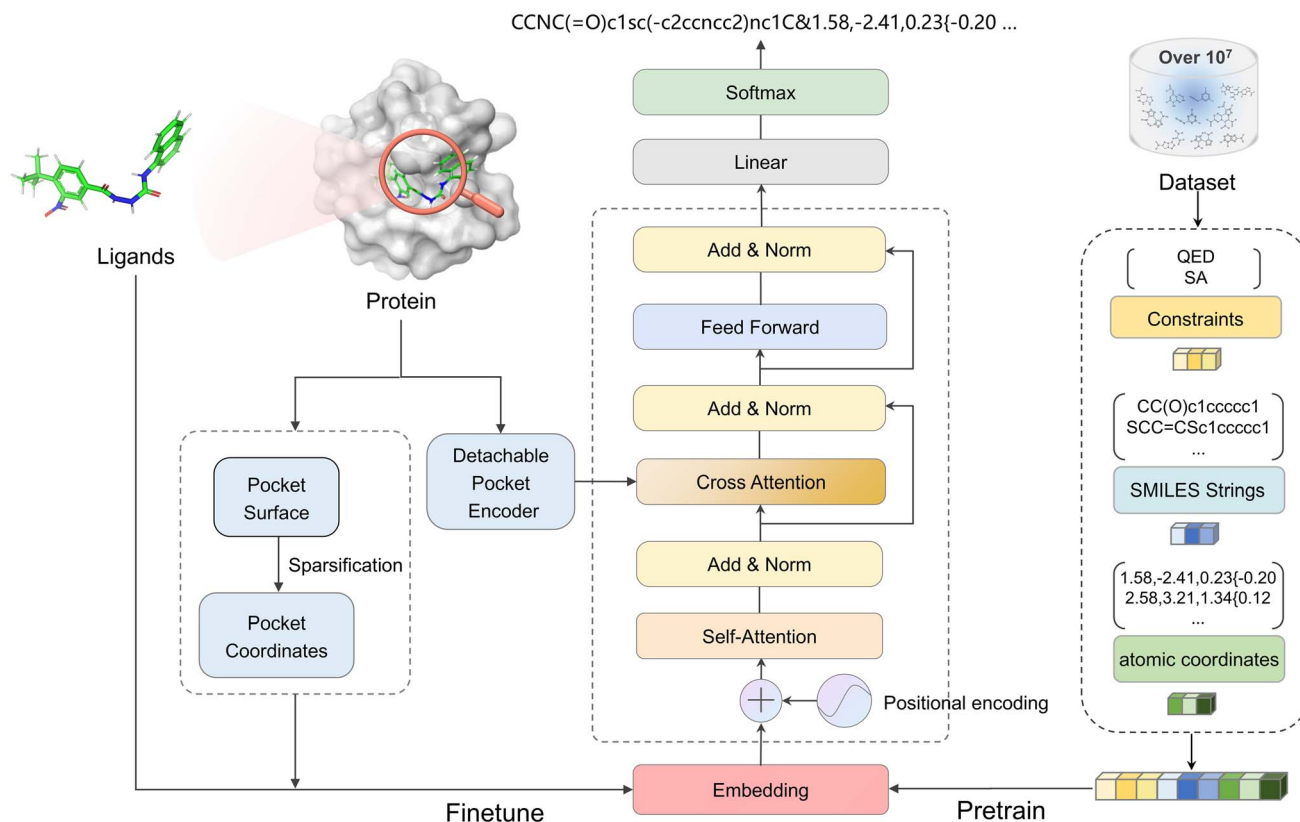
Fig. 1 The overview of 3DSMILES-GPT.
