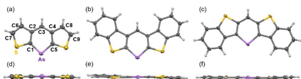
Fig. 2 ORTEP of (a and d) 3a , (b and e) 3c , and (c and f) 3d . Thermal ellipsoids are drawn at the 50% probability level.
