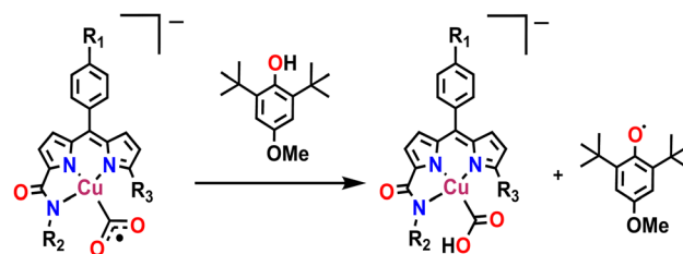
Scheme 2 Trapping the radical intermediate by HAT.
