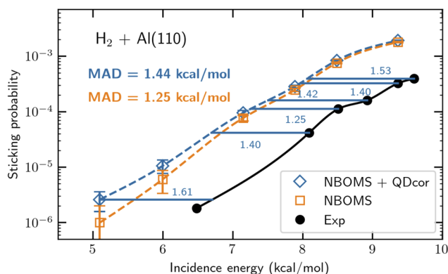
Fig. 13 Computed 37 and measured 241,242 S_0 for \text{H}_2 + \text{Al}(110) . S_0 computed with the NBOMS model, and as computed with the NBOMS model but also corrected for quantum dynamical effects, are compared to experimental values. The blue horizontal lines and numbers ( \text{kcal mol}^{-1} ) indicate the energy distance between the measured S_0 and the S_0 computed with the NBOMS model corrected for nuclear quantum effects. Figure taken from ref. 37 ( https://doi.org/10.1021/acs.jpcclett.3c02972 ). Further permission requests to be directed to the ACS.
