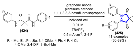
Scheme 113 Synthesis of 1,2-diarylpyrazolidin-3,5-diones via electrochemical method.
