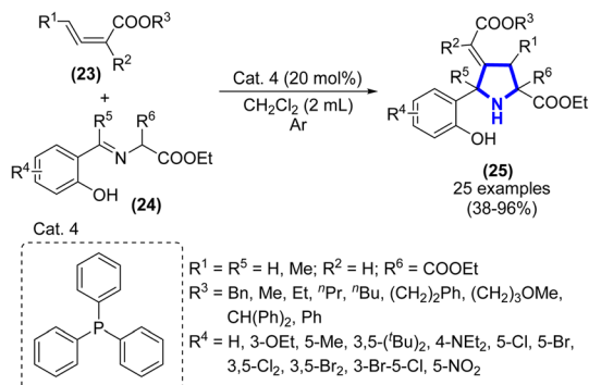
Scheme 6 Synthesis of 4-methylenepyrrolidine derivatives catalyzed by Cat. 4.
