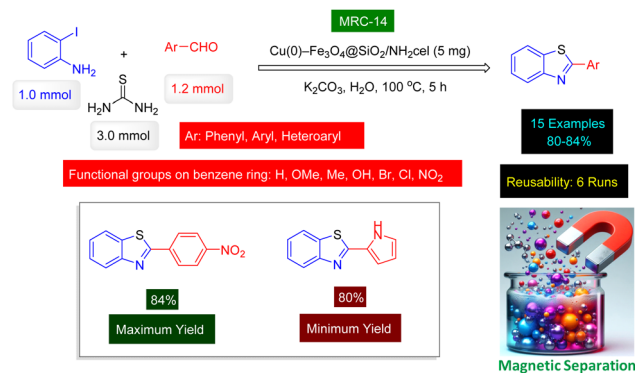
Scheme 14 \text{Cu}(0)\text{-Fe}_3\text{O}_4\text{@SiO}_2/\text{NH}_2\text{cel} nanomaterial (MRC-14) catalyzed preparation of 2-aryl benzothiazole derivatives from thiourea.
