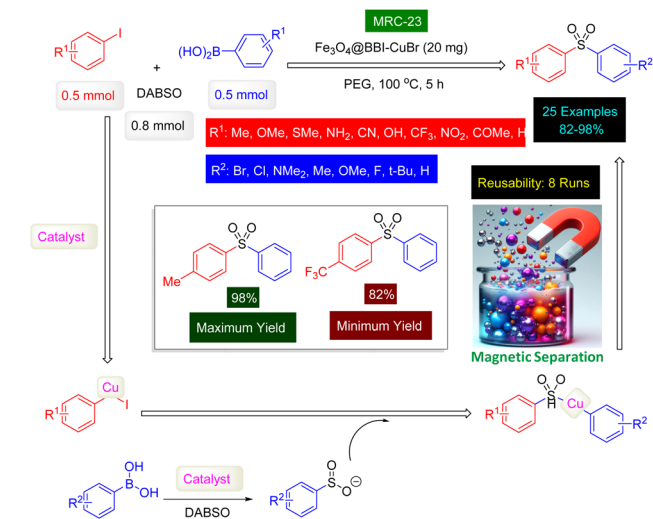
Scheme 23 \text{Fe}_3\text{O}_4@\text{BBI-CuBr} nanomaterial (MRC-23) catalyzed preparation of diaryl sulfone derivatives from DABSO.
