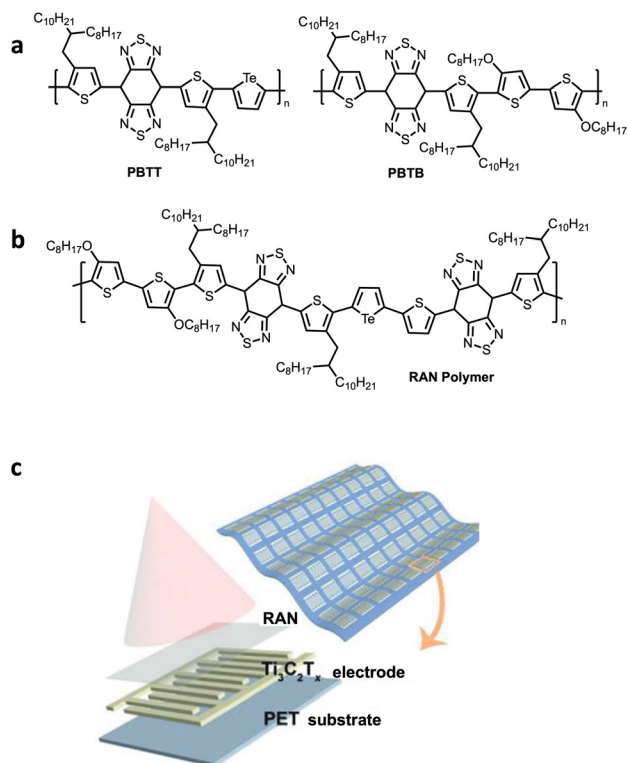
Fig. 24 Reports of telluophene-based polymers in OPD applications. (a) Polymeric structures of PBTT and PBTB used in short-wave infrared (SWIR) OPDs. (b) Structure of RAN polymer used in the NIR \text{Ti}_3\text{C}_2\text{T}_x -RAN PD. (c) Schematic diagram of single \text{Ti}_3\text{C}_2\text{T}_x -RAN PD structure. Reproduced from ref. 119 with permission from John Wiley and Sons, copyright 2022.
