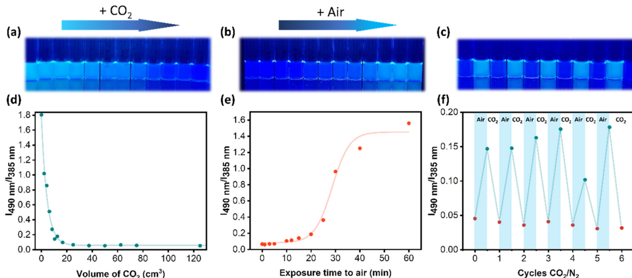
Fig. 3 (a) Photograph of P(DMAm-co-DEAPyMA) samples of concentration 0.01 \text{ mg mL}^{-1} after bubbling different CO 2 volumes (OFF process) under 365 nm UV light. (b) Photograph of P(DMAm-co-DEAPyMA) samples of concentration 0.01 \text{ mg mL}^{-1} after being exposed to atmospheric air for 1 h (ON process) under 365 nm UV light. (c) Photograph of P(DMAm-co-DEAPyMA) samples of concentration 0.01 \text{ mg mL}^{-1} after undergoing several CO 2 /air cycles under 365 nm UV light. (d) Kinetics graphic representing a change in fluorescence intensity ratio I_{490\text{nm}}/I_{385\text{nm}} of a sample of concentration 0.01 \text{ mg mL}^{-1} relative to the volume of CO 2 . (e) Kinetics graphic representing a change in fluorescence intensity ratio I_{490\text{nm}}/I_{385\text{nm}} of a sample of 0.01 \text{ mg mL}^{-1} concentration when exposed to air for 1 h. (f) Graphic representing the change in fluorescence intensity ratio I_{490\text{nm}}/I_{385\text{nm}} of a sample of concentration 0.01 \text{ mg mL}^{-1} when being exposed to CO 2 for 5 min and air for 1 h for 6 cycles.
