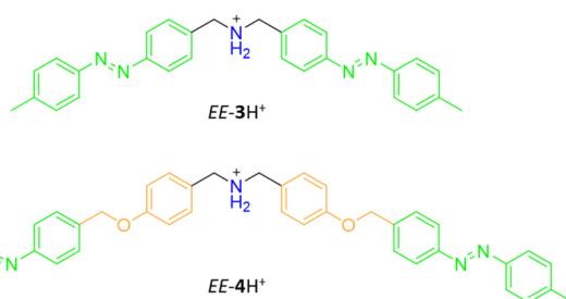
Fig. 2 Structure formula of the symmetric axes EE-3H^+ and EE-4H^+ .
