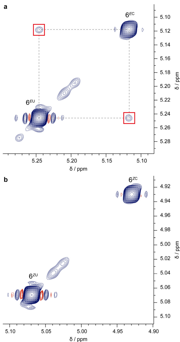
Fig. 5 Partial EXSY NMR ( CD_3CN , 500 MHz, 298 K, 1.4 mM, t_{\text{mix}} = 600 ms) spectra of (a) an equimolar mixture of EE\text{-}4H^+ and 2 , and (b) the same sample after exhaustive irradiation at 365 nm. 6^{EU} and 6^{EC} in (a) indicates the free and complexed EE axle, respectively, whereas 6^{ZU} and 6^{ZC} in (b) denote the free and complexed ZZ axle, respectively.
