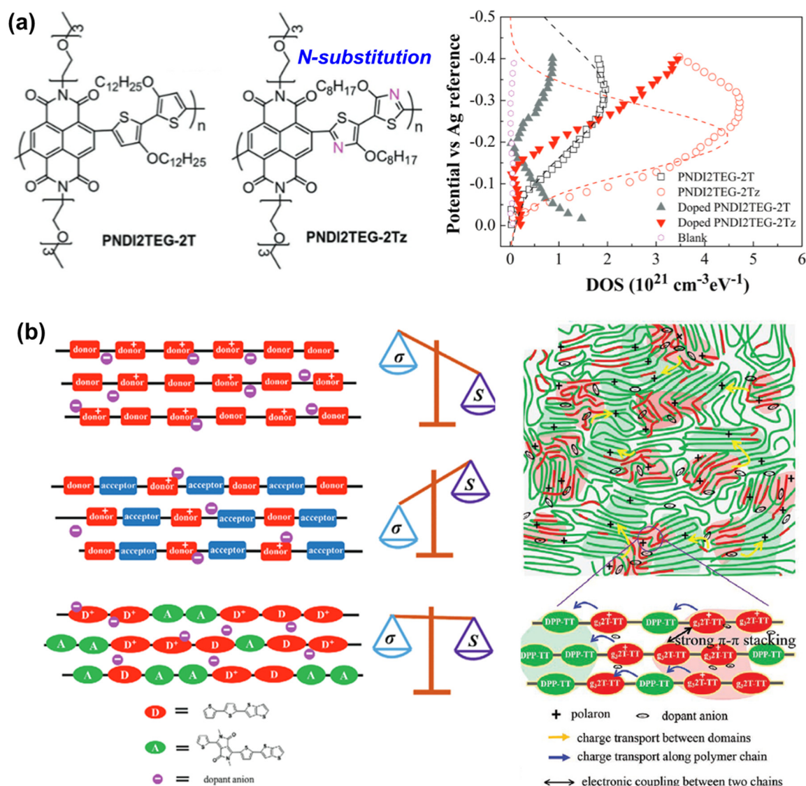
Fig. 4 (a) \text{sp}^2 N-substitution in the donor moiety makes the DOS of the donor–acceptor copolymer narrower (degenerate), which is ideal for maintaining a high \sigma and S 34 (reproduced with permission, Copyright 2018, Wiley-VCH). (b) Polymers with only donors have a high \sigma and low S , polymers with an alternate sequence of donors and acceptors have a high S due to interchain energetic disorder but low \sigma , whereas polymers with a random sequence of donors and acceptors have both high S and \sigma 21 (reproduced with permission, copyright 2020, Wiley-VCH).
