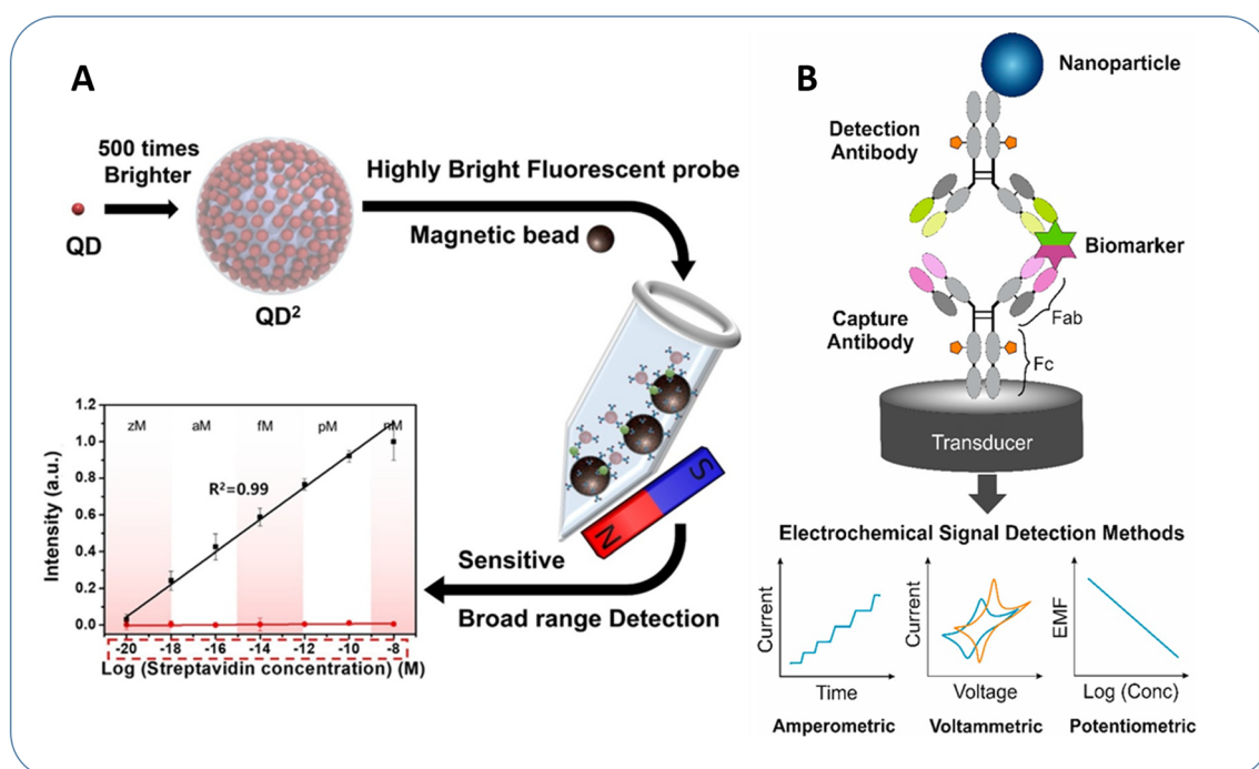
Fig. 4 (A) This image shows a highly bright fluorescent probe ( \text{QD}^2 ) with 500 \times brighter quantum dots on magnetic beads, enabling ultra-sensitive detection across a wide range (zeptomolar to nanomolar) with R^2 = 0.99 . Ideal for precise and sensitive analyte detection. This figure has been adapted from ref. 86 with permission from Elsevier, copyright 2020. (B) Schema of electrochemical immunosensors based on nanoparticle tags. This figure has been adapted from ref. 87 with permission from MDPI AG, copyright 2021.
