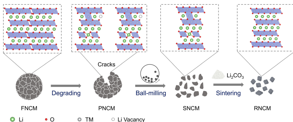
Fig. 6 Schematic illustration of the direct regeneration of mechanically degraded NCM70.
