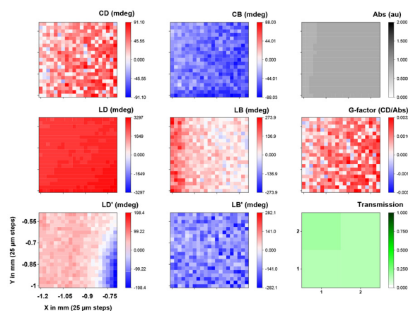
Fig. 8 Optical activity MMP maps at 600 nm of a 0.5 × 0.5 mm area (21 × 21 steps) with a lateral resolution of 25 μm of a blade coated film of ( S,S )-1 : ITIC-4F on ITO-functionalized glass slide.
