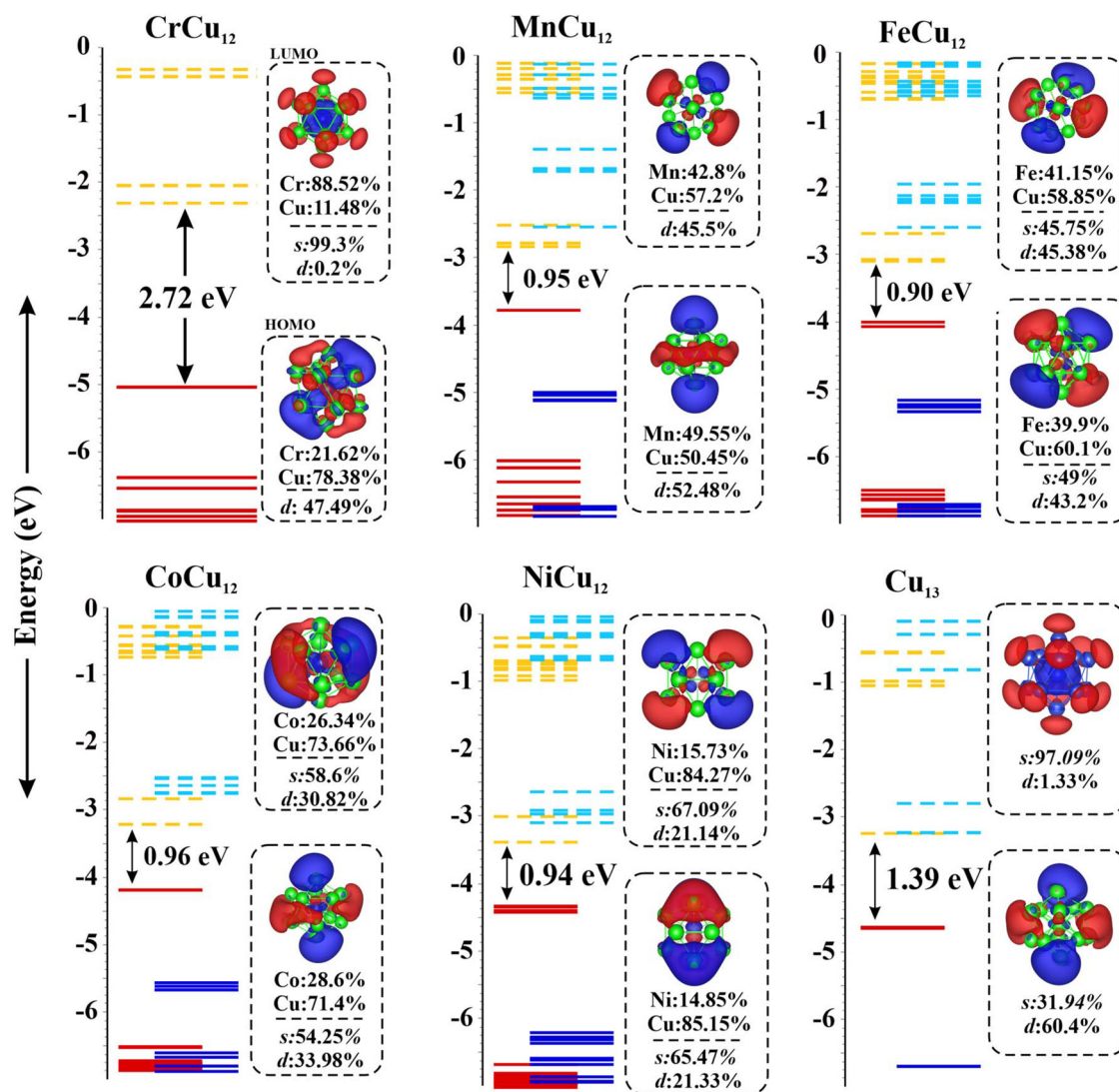
Fig. 2 Molecular orbital maps of HOMO and LUMO of the Cr/Mn/Fe/Co/Ni/Cu- \text{Cu}_{12} clusters; solid and dashed lines represent occupied and unoccupied states.
