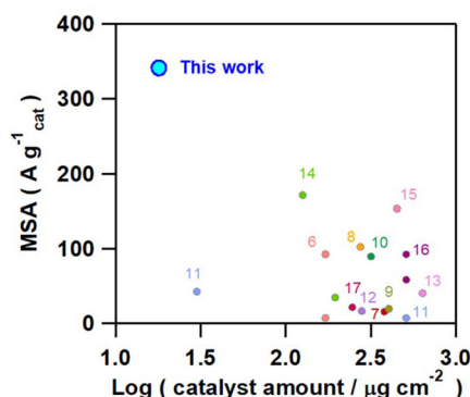
Fig. 1 Relationship between mass-specific activity (MSA) and catalyst-loading amount (circles) of the RuO 2 electrodes reported so far for OER under acidic conditions. Blue circle expresses the data of the present study. The number expresses the reference numbers in the text.
