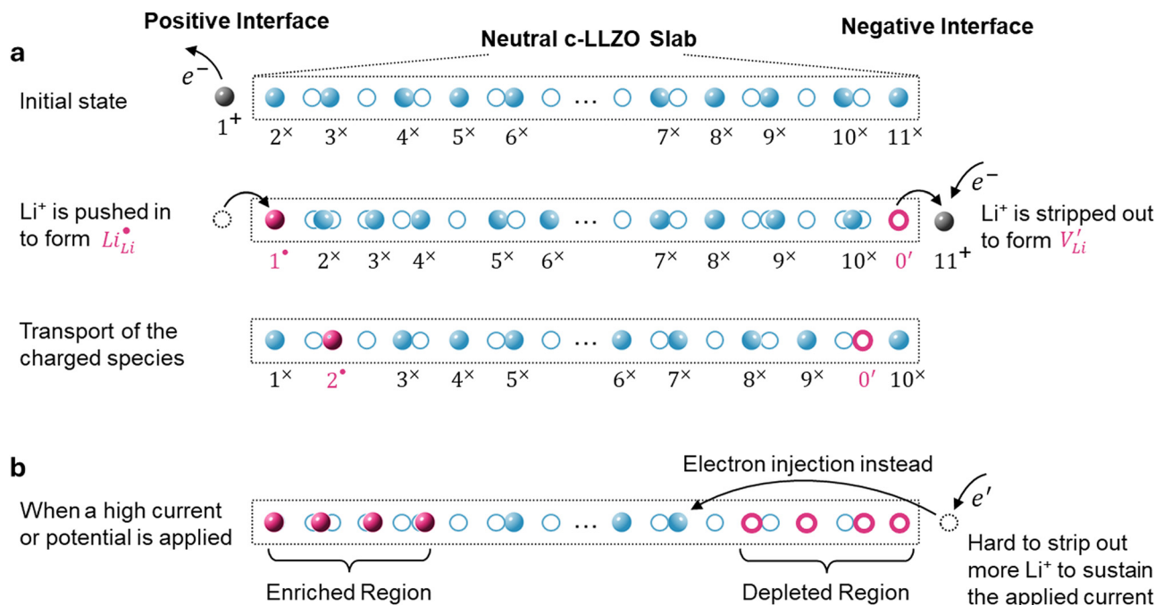
Fig. 3 Schematic explanations of (a) the generation and transport of \text{Li}_{\text{Li}}^\bullet at the positive interface and V_{\text{Li}}' at the negative interface in a single Li-ion conducting channel, due to the electrochemical transfer of \text{Li}^+ ions across the interfaces; and (b) the scenario of the generation and accumulation of \text{Li}_{\text{Li}}^\bullet and V_{\text{Li}}' in high-current conditions.
