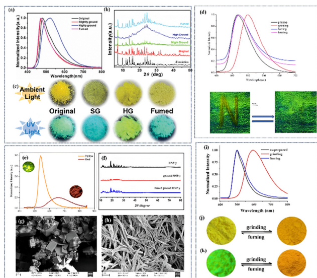
Fig. 3 Mechanoluminescence properties of \text{Zn}(\text{II}) complexes based on Schiff base \text{ML}^3 (a) and (c) Fluorescence emission spectra and appearance of the sample under ambient and UV light, (b) PXRD pattern; reproduced from ref. 70 with permission from RSC, Copyright 2021; (d) fluorescence spectra at 420 nm in different solid states upon grinding and fuming/heating of \text{HL}^4 ; reproduced from ref. 56 with permission from Elsevier, Copyright 2019; (e) orange and red line fluorescence spectra of the naphthaldehyde Schiff base of powdered \text{H}_4\text{L}^2\text{-y} and \text{H}_4\text{L}^2\text{-r} , respectively, (f) PXRD patterns of \text{H}_4\text{L}^2\text{-y} and \text{H}_4\text{L}^2\text{-r} crystals when ground and fumed with DCM, (g) and (h) SEM image of \text{H}_4\text{L}^2 ; reproduced from ref. 57 with permission from RSC, Copyright 2022; (i) of \text{HL}^5 showing normalized fluorescence spectra in different solid-states, ground and fumed at 365 nm (j) and (k) solid colour appearance of \text{HL}^5 under ground and fumed conditions; reproduced from ref. 73 with permission from Elsevier, Copyright 2019.
