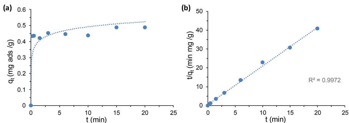
Fig. 6 (a) Hg(II) absorption kinetics of Zr-MSA-UV2 for 20 minutes contact. (b) The pseudo-second-order kinetic plot for the absorption (Hg(II) concentration of 10 mg L -1 ).
