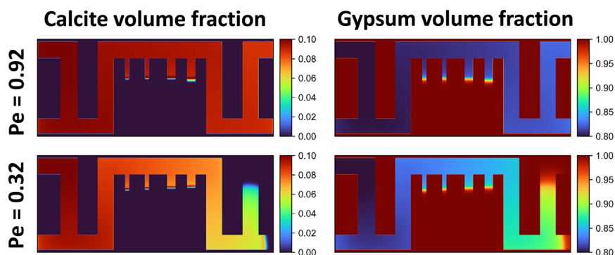
Fig. 8 Calcite and gypsum volume fraction on a sidewall at 0.6 days for Pe = 0.92 and 0.32 .
