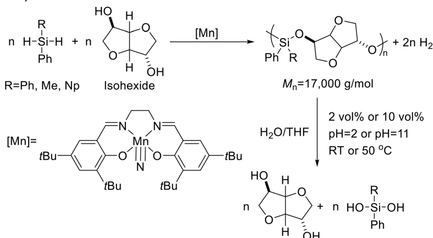
Fig. 20 Synthesis of bio-based poly(silyl ether)s from hydrosilanes and isohexide. 28
