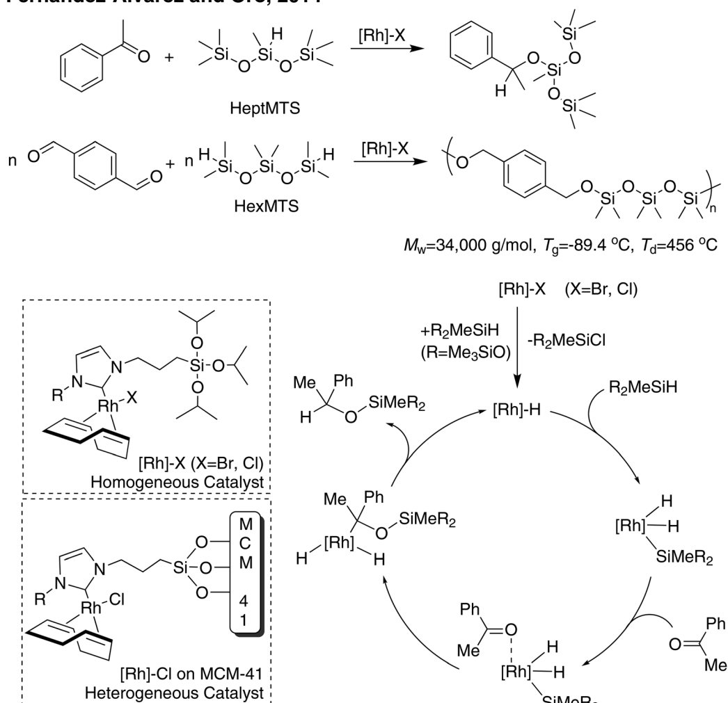
Fig. 12 Hydrosilylation polymerization of terephthalaldehyde and HexMTS catalyzed by Rh-based catalysts, along with the plausible mechanism. 40
