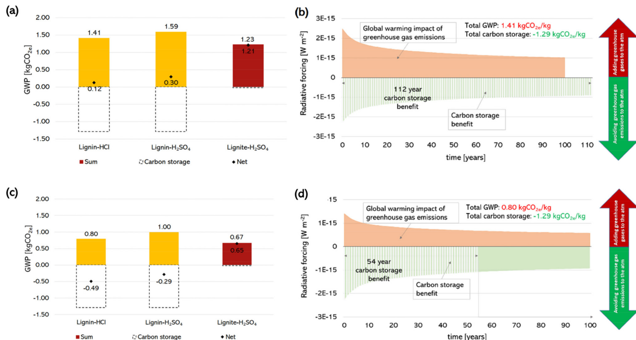
Fig. 3 Life cycle assessment. (a) Global warming potential results for 1 kg of composite panel for the lignin-HCl, lignin-H 2 SO 4 , and lignite-H 2 SO 4 base case scenarios, respectively. (b) Life cycle greenhouse gas emissions and carbon storage benefits using a temporal radiative forcing analysis for the base case scenario for lignin-HCl. (c) Global warming potential results for 1 kg of composite panel in alternative scenarios (100% recycled HDPE and renewable electricity) for the lignin-HCl, lignin-H 2 SO 4 , and lignite-H 2 SO 4 cases, respectively. (d) Life cycle greenhouse gas emissions and carbon storage benefits using temporal radiative forcing analysis for the alternative scenario for lignin-HCl.
