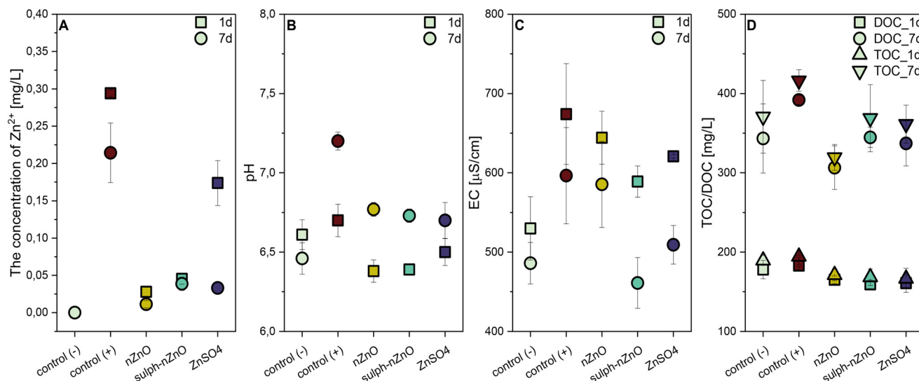
Fig. 3 \text{Zn}^{2+} concentrations (A), pH (B), EC (C), and DOC and TOC (D) in the growth medium of barley following exposure to Zn compounds for 1 and 7 days. The control (–) and the control (+) mean the untreated plants grown in HGL solutions without or with Zn ions (as \text{ZnSO}_4 ), respectively. Error bars represent standard error ( n = 3 repeats).
