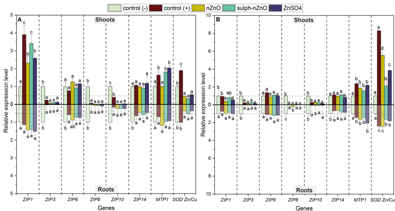
Fig. 9 The relative expression of genes related to Zn homeostasis in barley roots and shoots exposed for 1 (A) and 7 days (B) to nZnO, sulph-nZnO, and ZnSO 4 . The control (-) and the control (+) mean the untreated plants grown in HGL solutions without or with Zn ions (as ZnSO 4 ), respectively. Error bars represent standard error ( n = 3 biological repeats). Different letters indicate significant differences among the treatments (Tukey test, p < 0.05 ).
