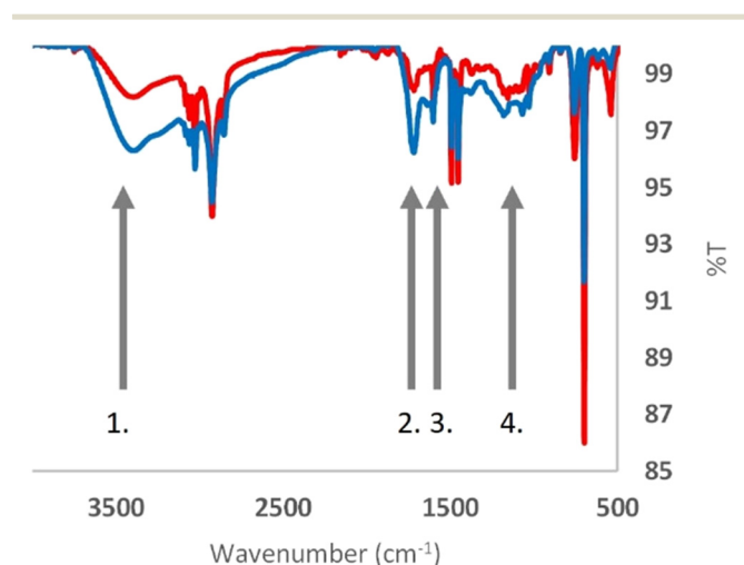
Fig. 3 UATR-FTIR spectra for the 53 nm PS-NH 2 particles. Red is the control, placed in a glass Petri dish during the experiment, sample. Blue is the UV-B treated, placed in a quartz Petri dish during the experiment, sample. The grey arrows indicate some of the changes in the FTIR spectra.
