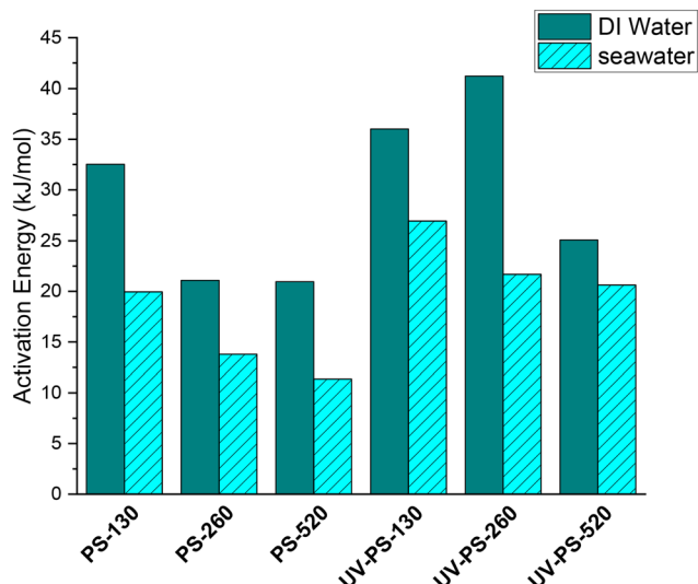
Fig. 7 Activation energy ( E_a ) of \text{Cu}^{2+} adsorption by original and UV-aged PS particles in DI water and seawater.
