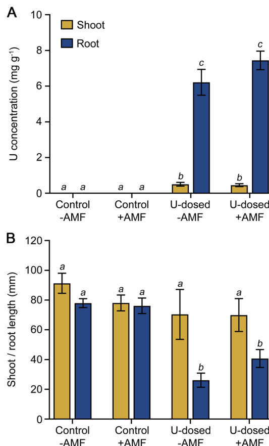
Fig. 1 U accumulation and plant growth response in control (undosed) and U-dosed non-mycorrhizal (–AMF) and mycorrhizal (+AMF) P. lanceolata seedlings. (A) Measurement of shoot and root U concentration. Control (background) U concentrations are all < 0.0002 \text{ mg g}^{-1} . (B) Measurement of shoot and root length. All data are mean values \pm SEM, n = 5 . Different lowercase letters indicate statistically significant differences ( P < 0.05 ) between samples. This indicates that U dosing was successful and that this elevated U content is the likely cause for decreased mean root length. AMF had no significant influence on shoot and root U content or shoot and root length.
