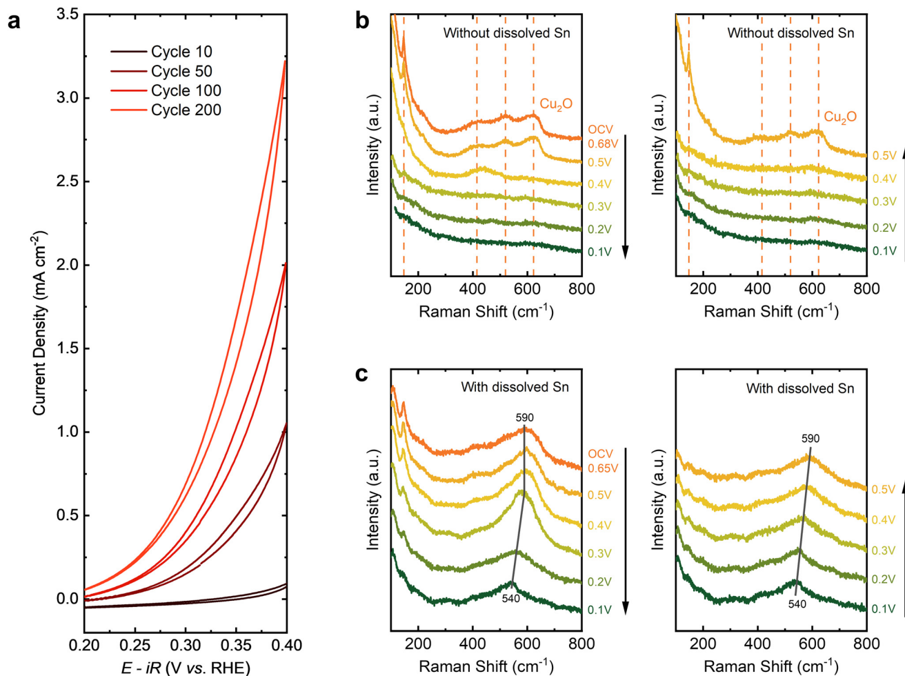
Fig. 4 (a) Cyclic voltammograms on Cu disk in Ar-saturated 1 M KOH + 50 mM \text{Sn(OH)}_3^- at 10 \text{mV s}^{-1} and 800 rpm. (b) In situ EC-Raman spectra on Cu nanoparticle electrode in Ar-saturated 4 M KOH. (Left) Polarization in the cathodic direction from pristine electrode. (Right) Subsequent polarization in the anodic direction. (c) In situ EC-Raman spectra on Cu nanoparticle electrode in Ar-saturated 4 M KOH and 0.1 M \text{Sn(OH)}_3^- (prepared with 4.1 M KOH and 0.1 M SnO). (Left) Polarization in the cathodic direction from pristine electrode. (Right) Subsequent polarization in the anodic direction. The electrode is scanned and held at each potential (vs. RHE) for at least 2 min before taking Raman measurements. Orange dashed lines: \text{Cu}_2\text{O} reference bands. 43,44 Gray solid lines: band assigned to surface \text{Sn(OH)}_x (guides to the eye).
