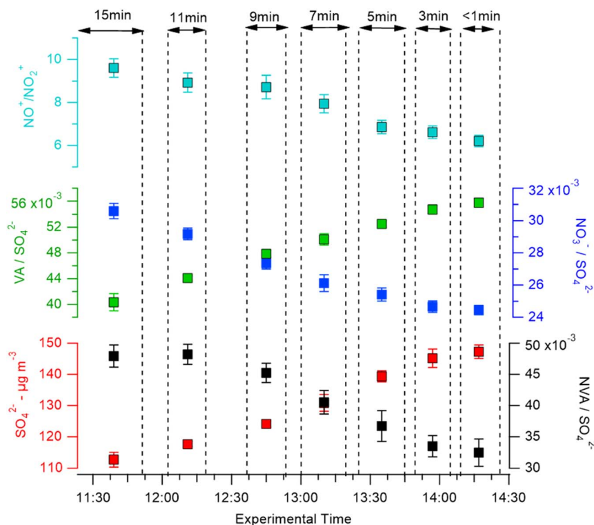
Fig. 2 Data collected during a typical experiment ( \text{RH} = 25\% ), where experimental time on the lower horizontal axis is the real time at which the measurements were conducted in the laboratory, plotted in the hh:mm format. The times on the upper horizontal axis ( i.e. , <1 to 15 min) correspond to the variable reaction times of \text{NO}_3 and particles in the flow tube, dependent on the injector position, where the first time bracket at 15 min represents the maximum exposure time, which decreases as the injector is pushed into the flow tube. Traces shown include aerosol sulfate ( \text{SO}_4^{2-} ), \text{NO}_3^+/\text{NO}_2^+ , and \text{SO}_4^{2-} -normalized vanillic acid (VA), nitrate (indicative of both inorganic and organic nitrates), and NVA.
