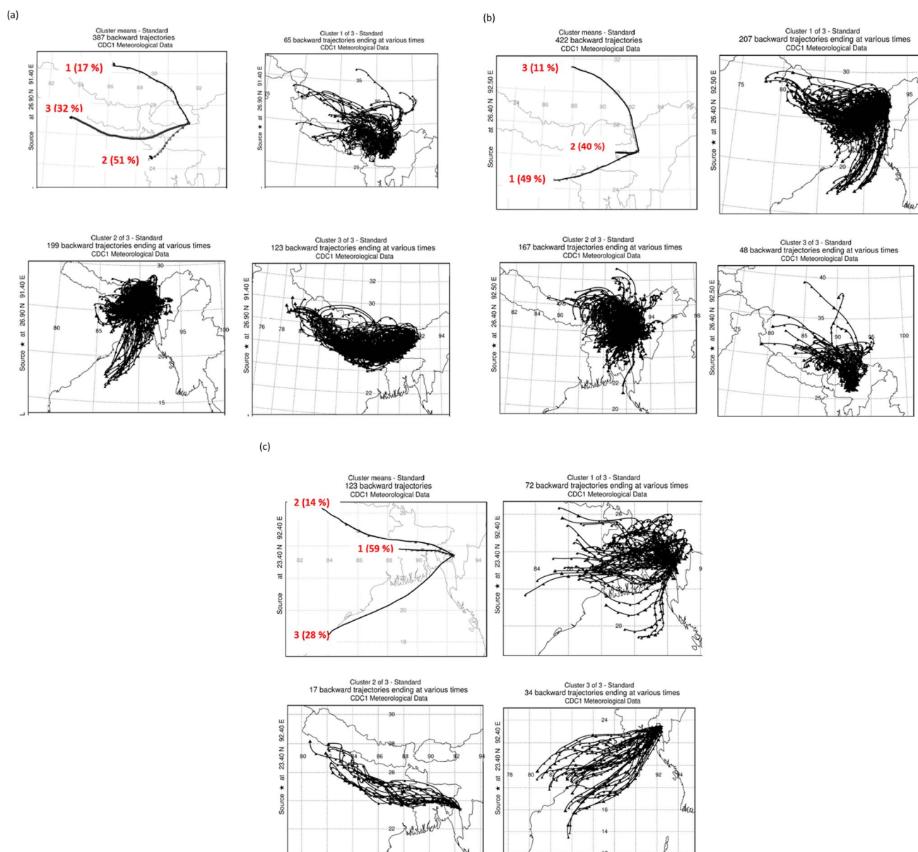
Fig. 5 72 h backward air mass trajectories arriving at 100 m agl during the FF >100 period at (a) Guwahati, (b) Tezpur and (c) Aizawl.
