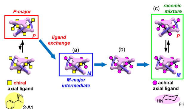
Fig. 17 Overview of the transient P/M chirality inversion observed during the racemization of L^5Co_3(S-A1)_6 via ligand exchange with piperidine.
