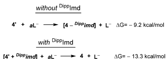
Scheme 5 Hypothetical ligand replacement reactions and the related free-energy changes.
