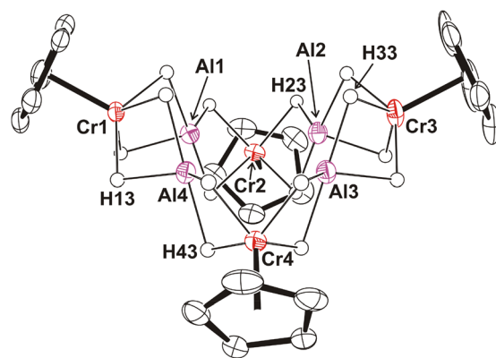
Fig. 5 Perspective view of 9 \cdot 1.5\text{C}_7\text{H}_8 with thermal ellipsoids at the 50\% probability level. Methyl groups of the \eta^5\text{-C}_5\text{Me}_5 ligands and toluene solvent molecules are omitted for clarity. Selected averaged lengths ( \text{\AA} ) and angles ( ^\circ ): Cr–H 1.63(5) , Al–H 1.72(2) , Cr–Cm 1.808(2) , Cr–Al 2.376(2) , \text{Cr}(1)/\text{Cr}(3)\cdots\text{Cr}(2) 4.748(2) , \text{Cr}(1)/\text{Cr}(3)\cdots\text{Cr}(4) 4.750(4) , \text{Cr}(2)\cdots\text{Cr}(4) 6.119(1) , Cr–Al–Cr 176(2) , Al–Cr–Al 78.2(3) , Cr–H–Al 90(2) , H–Cr–H 72(2)\text{--}88(2) and 131(2)\text{--}136(2) , H–Al–H 79(2)\text{--}102(2) , 121(2)\text{--}132(2) and 172(2)\text{--}178(2) .
