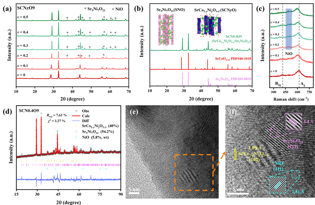
Fig. 1 (a) XRD patterns of \text{SCNxO9} ( x = 0-0.5 ). (b) XRD patterns of \text{SCN0.4O9} , \text{SrCoO}_{2.52} and \text{Sr}_9\text{Ni}_7\text{O}_{21} . (c) Raman spectra of \text{SCNxO9} ( x = 0-0.5 ). (d) Rietveld refinement results of the XRD pattern of \text{SCN0.4O9} . (e and f) TEM images of \text{SCN0.4O9} .
