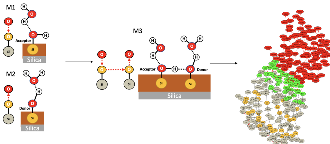
Fig. 11 Illustration of one 4-partner motif ( M3 ) made of the union of two 2-partner motifs ( M1 and M2 ) that are H-bonded together through silanol \cdots silanol. For one given snapshot taken randomly out of the 10 ps trajectory, the instances of M3 found at the (110)-quartz/liquid water interface are reported through the green vertices of the 2D-MolGraph (right side).
