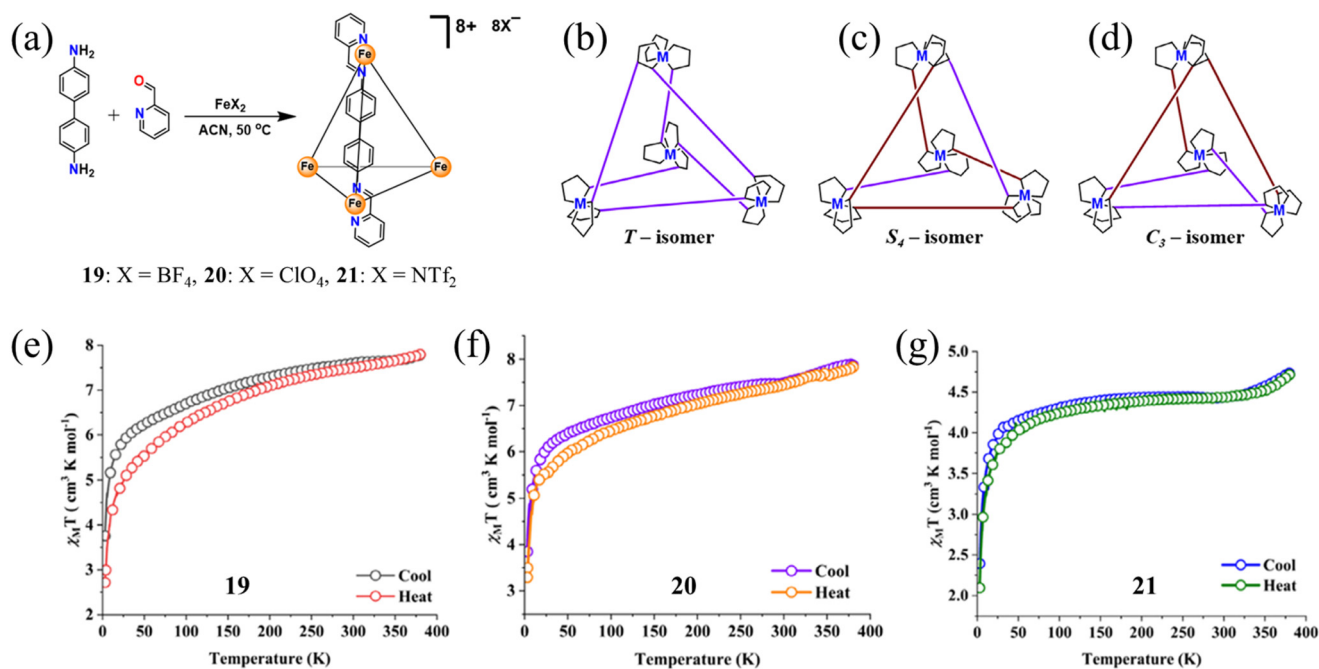
Fig. 17 (a) Synthesis method of cages 19–21 . (b–d) Diagrams of three diastereomers. \chi_{\text{M}}T vs. T plots for 19 (e), 20 (f) and 21 (g). Adapted from ref. 87.
