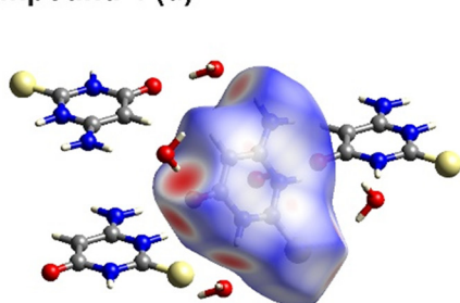
Fig. 5 Hirshfeld surfaces with short intermolecular contacts (red spots) in (a) 1, (b) 2, (c) 3, and (d) 4 (two perpendicular views). In the right column, 2D fingerprint plots of main contacts are represented.
