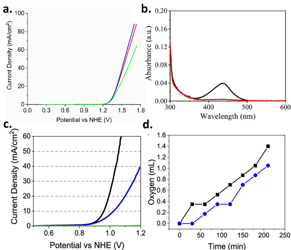
Fig. 4 Comparative analysis of electrodeposited chiral and achiral metal oxide films. (a) LSV plots of 500 nm thick L-CuO (shown as red line) and D-CuO (shown in blue line) film electrodes, with achiral glycine-CuO films (light green) showing reduced activity with respect to the chiral films. (b) UV-vis absorption spectra of the 0.1 M \text{Na}_2\text{SO}_4 electrolyte after titration with o -tolidine using chiral CuO (presented as red line) and achiral CuO (presented as a black line) as the working electrode. (c) LSV plots showing OER performance of L- \text{CoO}_x (shown as black line), meso - \text{CoO}_x (shown as blue line), and bare FTO (green) in 0.1 M KOH. (d) Oxygen production measured with a Hoffman apparatus for L- \text{CoO}_x (black) and meso - \text{CoO}_x (blue) catalysts. Figures are adopted from ref. 6 and 20 with permission from American Chemical Society © 2019 and American Chemical Society © 2020.
