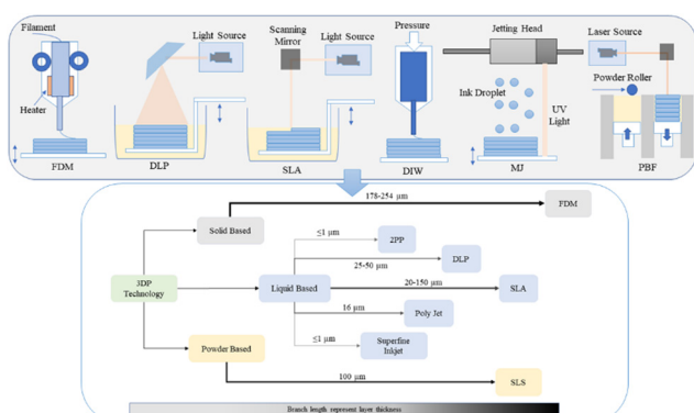
3D printing nomenclature: FDM: Fused deposition modelling; SLA: Stereolithography apparatus; DLP: Digital light processing; 2PP: two-photon polymerization; SLS: Selective layer sintering; MJ: Material jetting; PBF: Powder bed fusion
