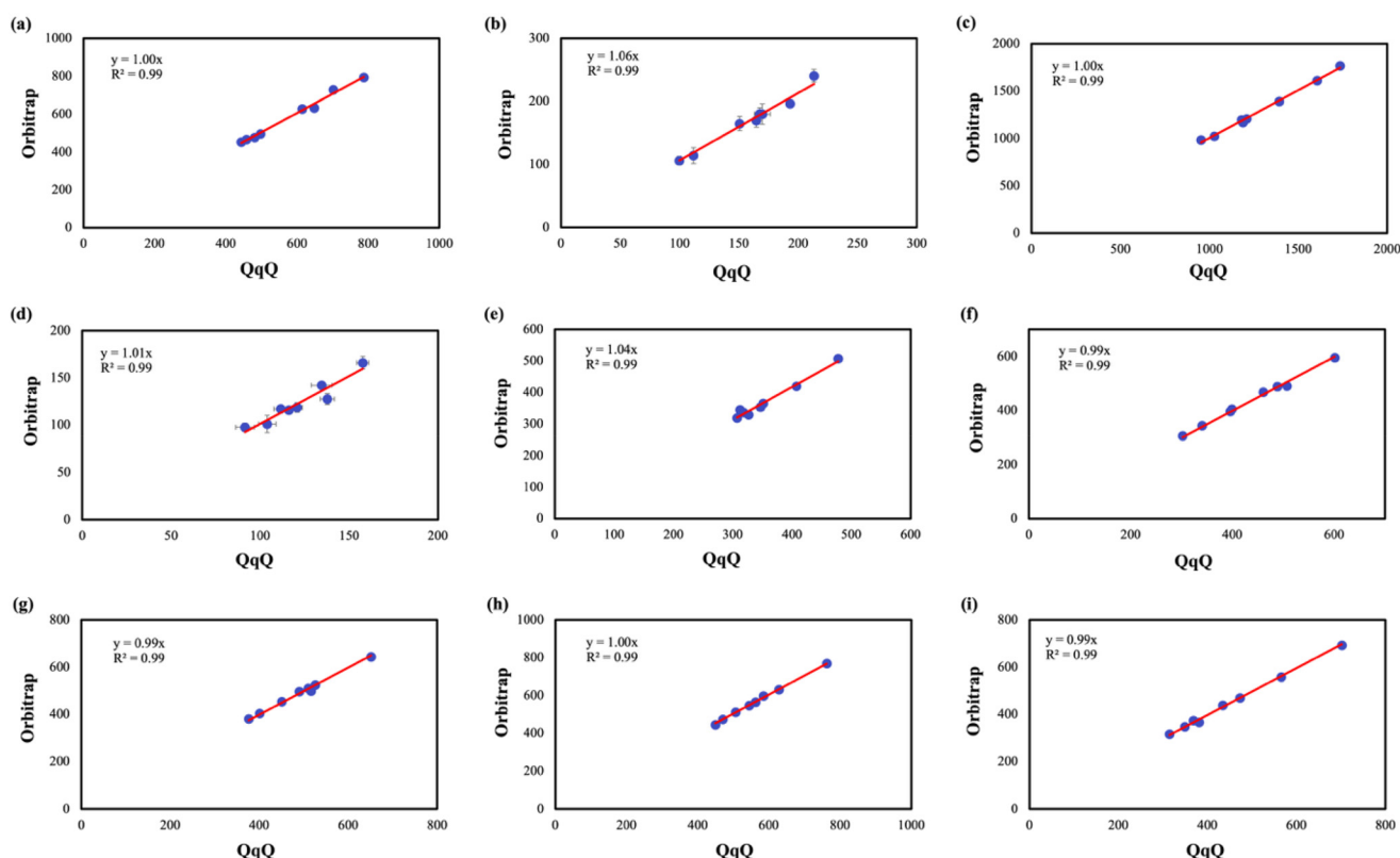
Fig. 4 Correlation plots comparing antibiotic concentrations (ng L -1 ) measured using LC-QqQ-MS and LC-Orbitrap-HRMS (a) ENF, (b) LIN (c) AZT, (d) OXC (e) SMZ (f) ERY (g) PEN (h) CIP and (i) LEV. *Red lines represent the linear regression fits. Slopes and R^2 values are displayed on each plot, indicating strong to excellent agreement across most analytes, with minor compound-specific deviations attributed to matrix effects and differences in quantification strategy. Horizontal and vertical error bars indicate the standard deviations of antibiotic concentration measured using LC-QqQ-MS and LC-Orbitrap-HRMS, respectively.
