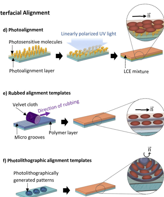
Fig. 7 LCE alignment methods: (1) bulk alignment: (a) electric field: the director aligns with the electric field direction. (b) Magnetic field: mesogens align with the magnetic induction intensity direction. (c) Mechanical stresses: alignment direction follows the stretching direction. (2) Interfacial alignment: (e) rubbed alignment templates: the direction of mechanical friction during rubbing defines the alignment direction of the mesogens. (f) Photolithographic alignment templates: microchannel direction dictates the alignment of mesogens within the LCE.
