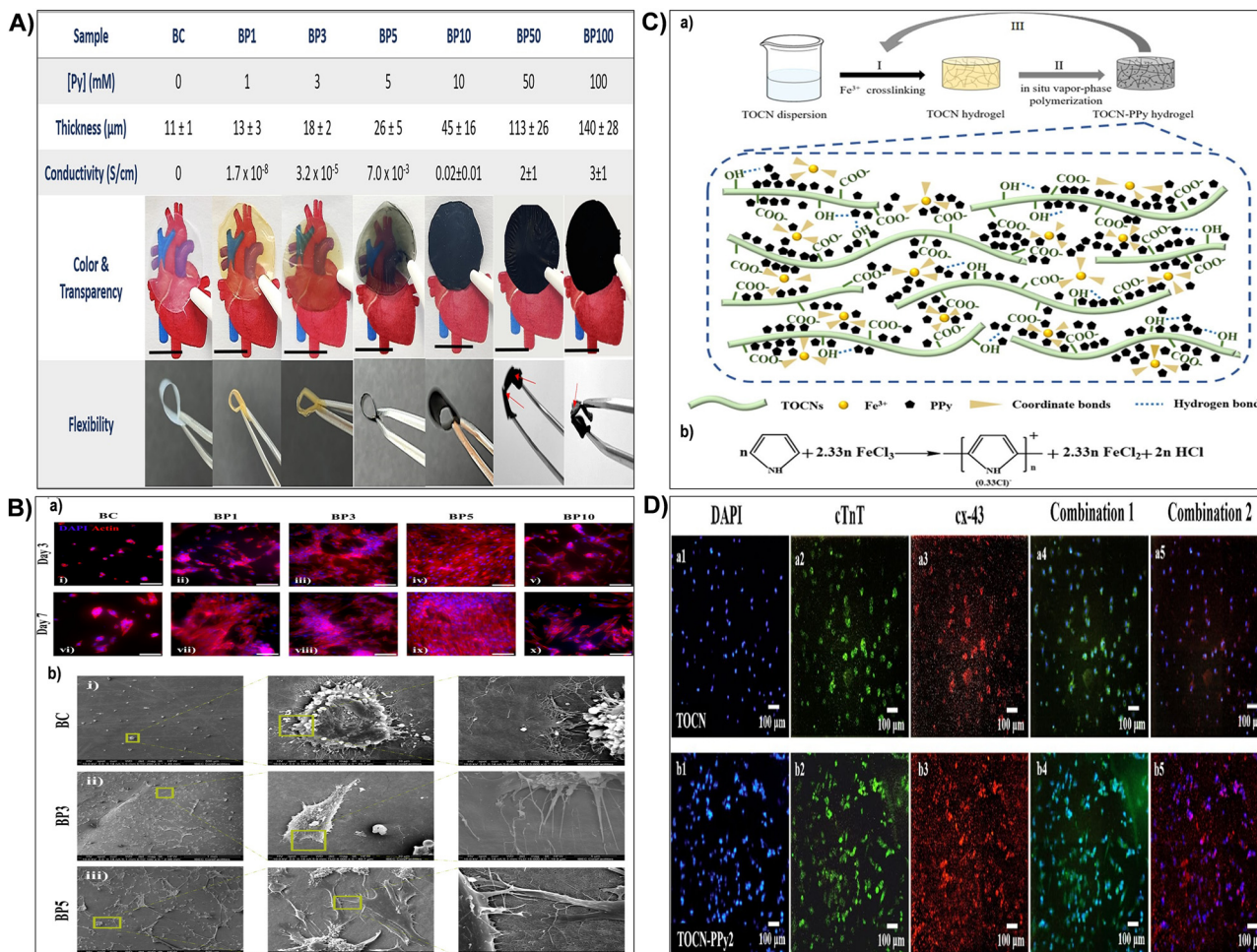
Fig. 25 (A) Impact of Py concentration on scaffold properties. Bacterial nanocellulose (BC) and bacterial nanocellulose-polyppyrrrole nanocomposites (BC-Ppy) at varying pyrrole (Py) concentrations and their property alterations. Scale bars: 1 cm. Reproduced with permission from ref. 540 Copyright © 2023 American Chemical Society. (B) H9c2 cell attachment to BC and BC-Ppy scaffolds. (a) Fluorescence microscopy images showing H9c2 cell populations on nanocellulose composites after 3 and 7 days of culture. Scale bars: 100 \mu\text{m} . (b) SEM images illustrating H9c2 attachment and morphology after 7 days of culture on BC, BP3, and BP5 materials. Reproduced with permission from ref. 540 Copyright © 2023 American Chemical Society. (C) Preparation process of nano-cellulose/polyppyrrrole conductive hydrogel. (a) Sequential cross-linking of TOCN dispersion with \text{Fe}^{3+} ions, followed by vapor-phase pyrrole monomer polymerization to form TOCN-Ppy1 composite hydrogel, repeated to generate TOCN-Ppy2 and TOCN-Ppy3 composite hydrogels. (b) Schematic representation of pyrrole polymerization with \text{FeCl}_3 . Reproduced with permission from ref. 541 Copyright © 2024 Springer. (D) Immunofluorescent staining of cells on pure TOCN and TOCN-Ppy2 hydrogels. DAPI (a1) and (b1), cTnT protein (a2) and (b2), cx-43 protein (a3) and (b3), (a4) combination diagram of a1 and a2, (a5) combination diagram of a1 and a3, (b4) combination diagram of b1 and b2, (b5) combination diagram of b1 and b3. Reproduced with permission from ref. 541 Copyright © 2024 Springer.
