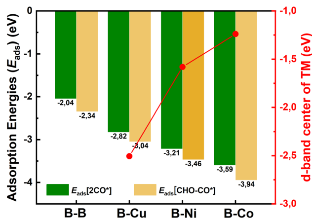
Fig. 6 Adsorption energies ( E_{ads} ) of 2CO^* and CHO-CO^* species on B-B@Si, B-Cu@Si, B-Ni@Si and B-Co@Si; and d-band centers of TM in bare hetero-B-TM@Si structures.
