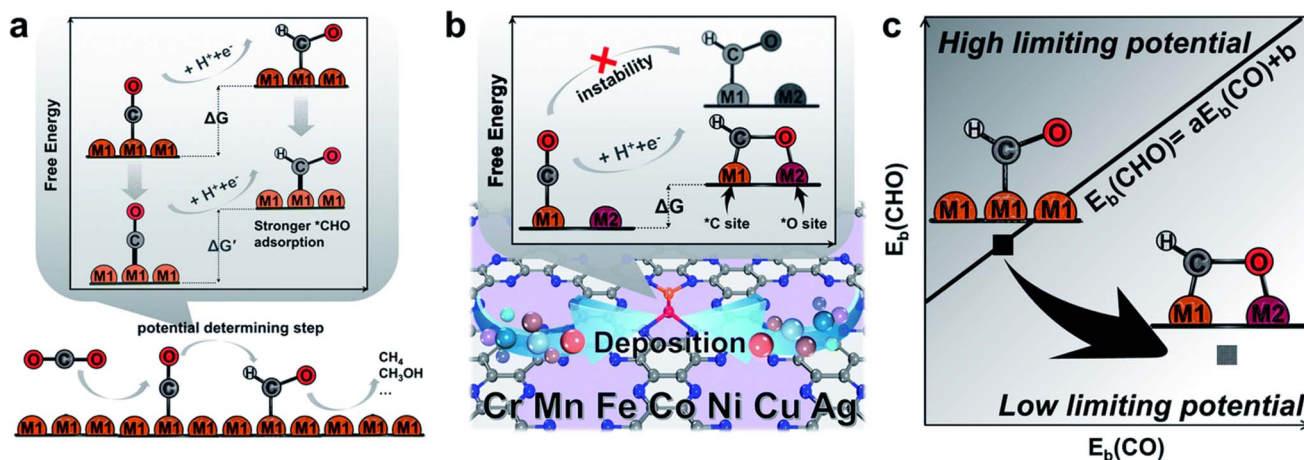
Fig. 1 (a) Effect of free energy change caused by the scaling relations between \text{CO} and \text{CHO} . (b) \text{C}_2\text{N} supported heteronuclear transition-metal dimers in stabilizing \text{CHO} . (c) The scaling relations between adsorption energies of \text{CHO} and \text{CO} . 30
