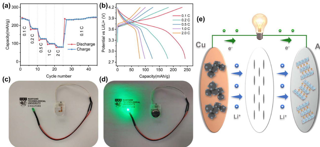
Fig. 7 (a) Rate capacities and (b) charge/discharge curves at different rates of LFNM-CuZn||LiNi 0.6 Co 0.2 Mn 0.2 O 2 full cells. (c and d) Photographs of a 3 V LED connected without/with the full cell. (e) Scheme of the LIB full cell.
