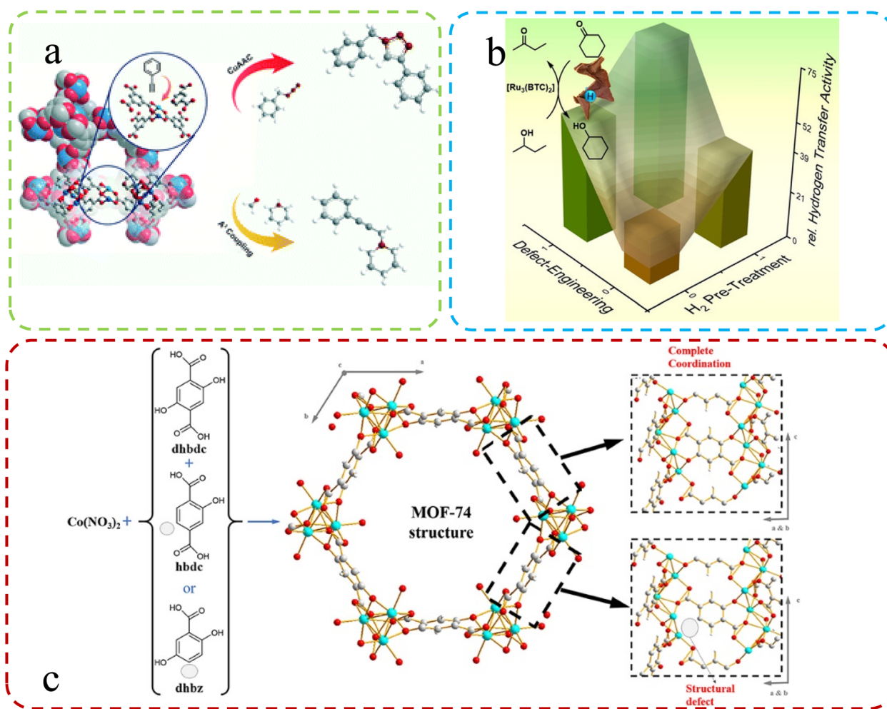
Fig. 3 (a) Schematic illustration of the mixed-linker approach. Reproduced with permission. 60 Copyright, 2021, Royal Society of Chemistry. (b) Defective HKUST-1 synthesized via the mixed-linker approach. Reproduced with permission. 54 Copyright, 2020, Wiley-VCH. (c) Generation of structural defects in a MOFs-74 structure by partial linker substitution. Reproduced with permission. 62 Copyright, 2019, Frontiers.
