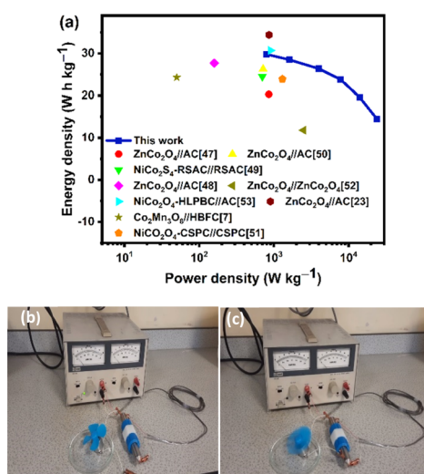
Fig. 8 (a) Ragone plot of the \text{ZnCo}_2\text{O}_4/\text{PPAC-4} asymmetric supercapacitor compared with other reported binary metal oxide//activated carbon asymmetric supercapacitor devices reported in the literature; practical application of the \text{ZnCo}_2\text{O}_4/\text{PPAC-4} asymmetric supercapacitor. (b) Device being charged at 1.6 V with power supply. (c) Performance of a motor/fan connected to the asymmetric supercapacitor.
