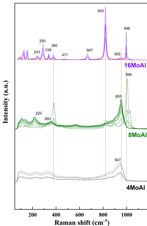
Fig. 2 Raman spectra of the synthesized catalysts (Mo-γ-Al 2 O 3 ) under ambient conditions.
