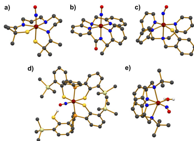
Fig. 2 Crystal structures of Fe–NO complexes, (a) [FeS 2 Me 2 N 3 (Pr,Pr)(NO)] + (7), (b) [Fe(MePcPy 3 )(NO)] 2+ (10), (c) [Fe(N3PyS)(NO)] + (13), (d) [Fe(TMSPS2)(TMSPS2H)(NO)] (16), and (e) [Fe(TBDAP)(NO)(H 2 O)] 2+ (20) (dark grey, C; blue, N; red, O; yellow, S; scarlet, Fe).
