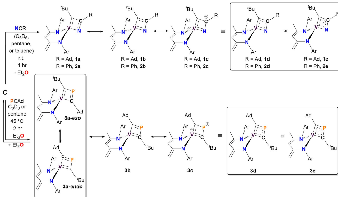
Scheme 1 Synthesis of complexes 1–3 via the [2+2]-cycloaddition of the vanadium alkylidyne C with pnictogen-containing alkynes \text{Pn}\equiv\text{CR} (Pn = N, R = Ad or Ph; Pn = P, R = Ad). Potential resonance structures and charge delocalized structures for each complex are also illustrated.
